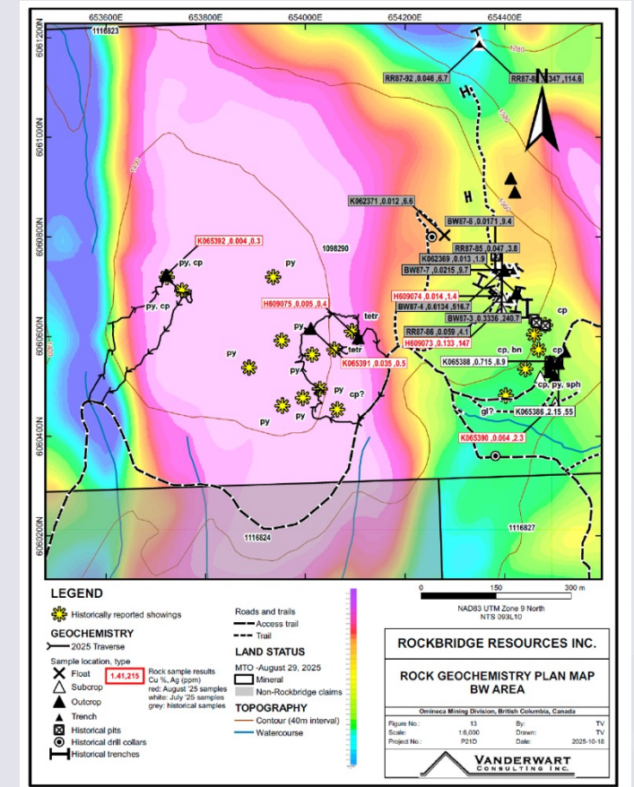
BW Target Area - Rock Geochemistry by Rockbridge 2024-2025
