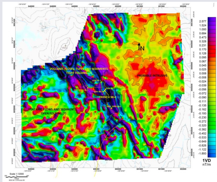
Del Santo Target First Vertical Derivative Magnetic Map
